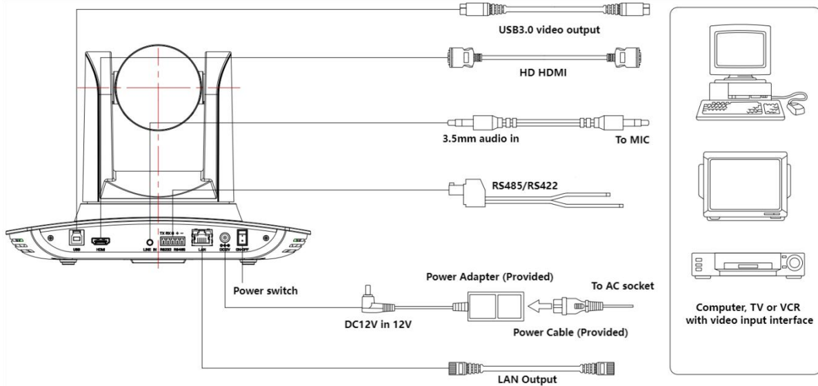
Figure 1.2 Wiring Diagram
